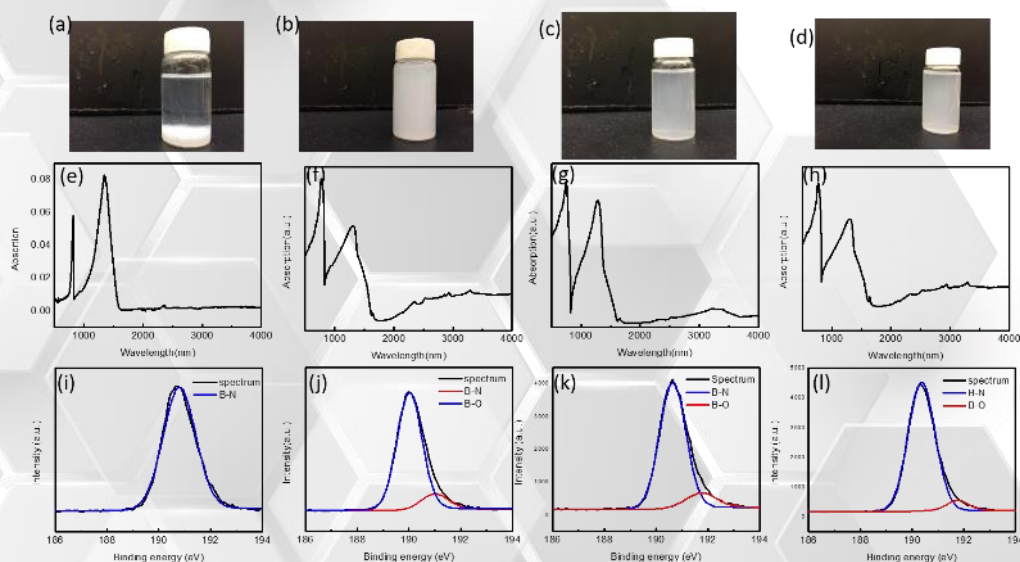
Figure3. h-BN functionalization with different functional groups. (a-d) suspension of h-BN, h-BN-OH, h-BN-NH 2 , h-BN-COOH. (e-h) FTIR spectra of h-BN, h-BN-OH, h-BN-NH 2 , h-BN-COOH. (i-l) XPS of B element of h-BN, h-BN-OH, h-BN-NH 2 , h-BN-COOH.
