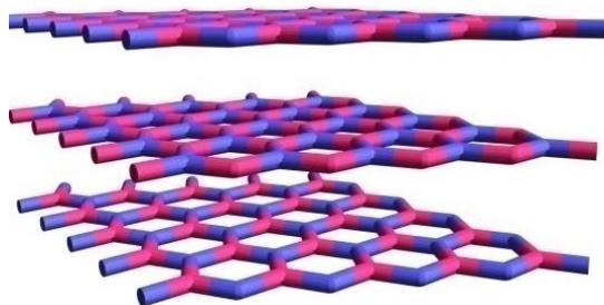
Boron Nitride
