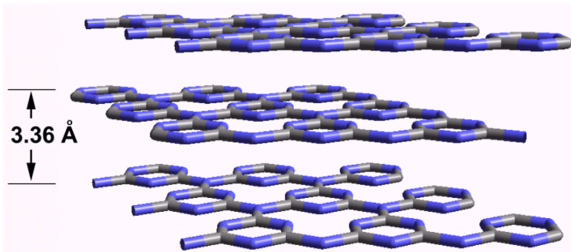
Carbon Nitride
