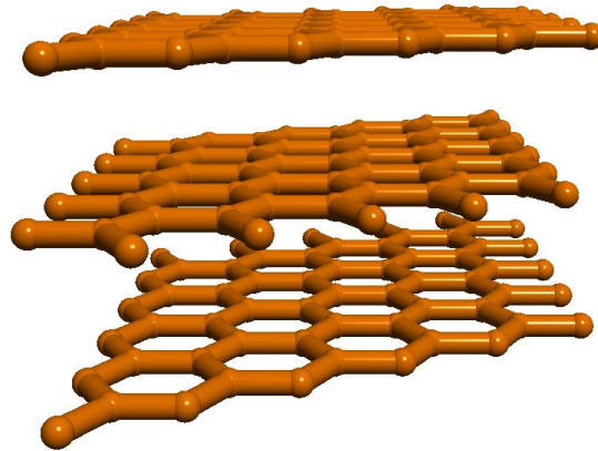
Graphite
