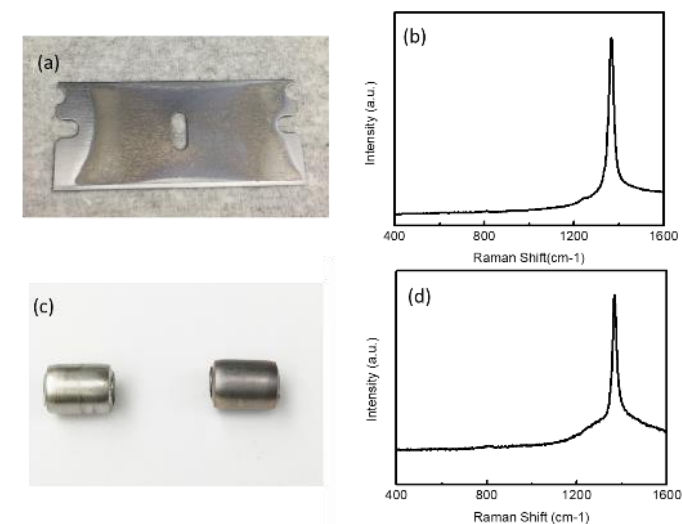
Figure2. CVD grown h-BN on carbon steel and stainless steel tube. (a-b) optical images and Raman of h-BN grown on carbon steel. (c-d) optical images and Raman of h-BN grown on stainless steel tube.
