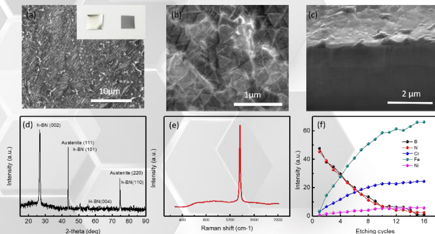
Figure1. CVD grown h-BN on stainless steel. (a-b) SEM images, inset is optical images before and after h-BN growth. (c) cross-section images of h-BN coated stainless steel. (d-f) XRD, Raman, and XPS depth profile of h-BN on stainless steel.
