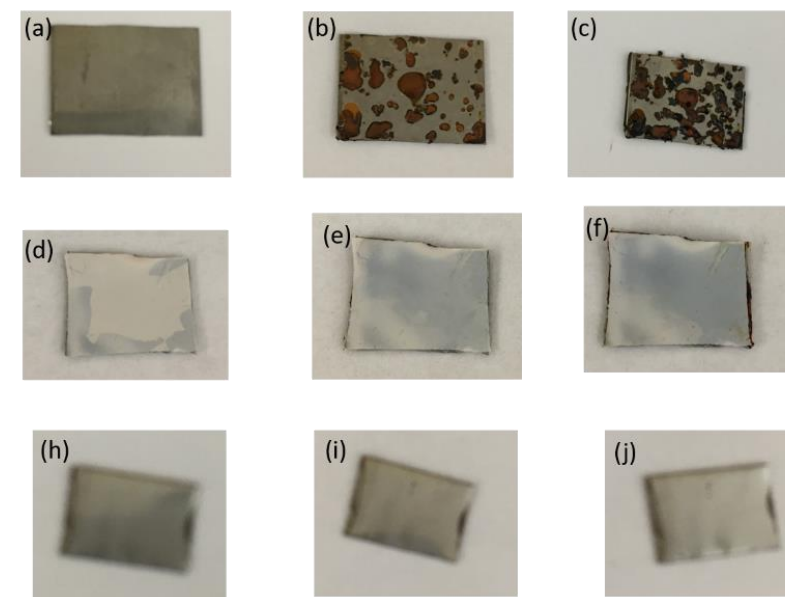
Figure4. Optical images of salt-spray tested samples. (a-c) bare carbon steel images for 0,1,2 days testing. (d-f) h-BN/PVDF coated carbon steel images for 0,1,2 days testing. (h-i) CVD grown h-BN on carbon steel images for 0,1,2 days testing.
