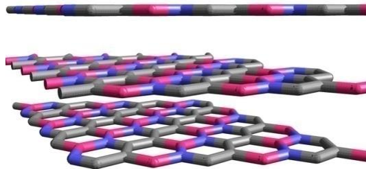
Boron Carbo-Nitride
